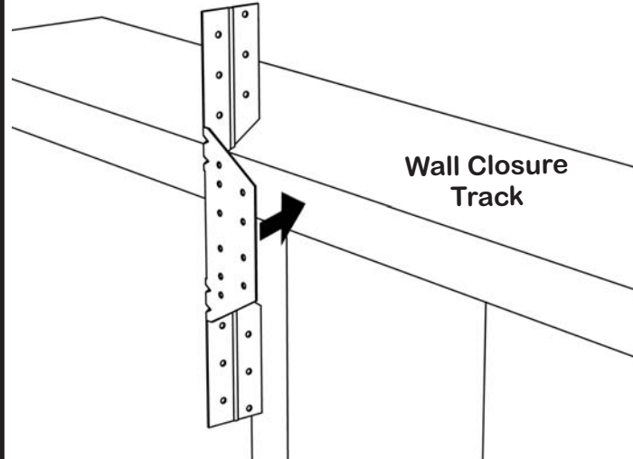
StiffClip® RT1300
