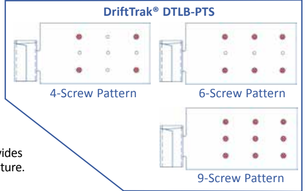
Fastener Patterns
