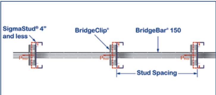
Bridging Load Bearing Studs Against Weak Axis Buckling
