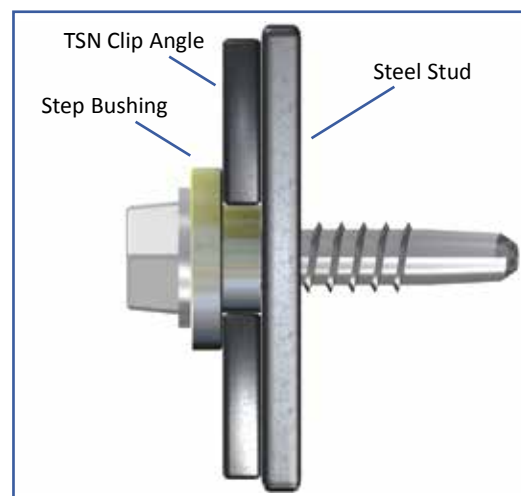
Step Bushings are seated inside slots of the VertiClips. Since Step Bushings are slightly thicker than the steel material, they provide a positive mechanical attachment to the stud web and allow for deflection movement.
