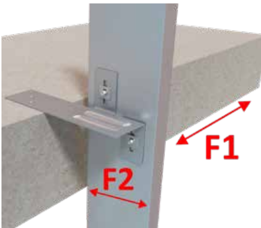
Load Direction
